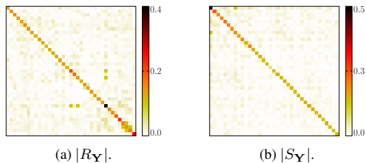
Fig. 4: Empirical spectral correlation matrices of \mathbf{Y} .
