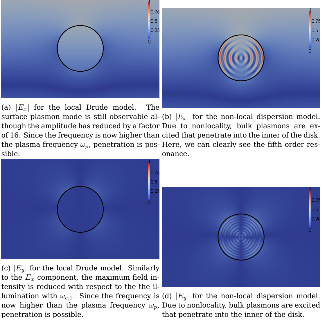
Figure 14: Field solutions of a dispersive nanodisk with a radius of 2 nm. The four figures show the Fourier transformed field solutions of |E_x| and |E_y| for the local and non-local dispersion model. All computations were done with DGTD- \mathcal{P}_2 at \omega_{c,2} .
