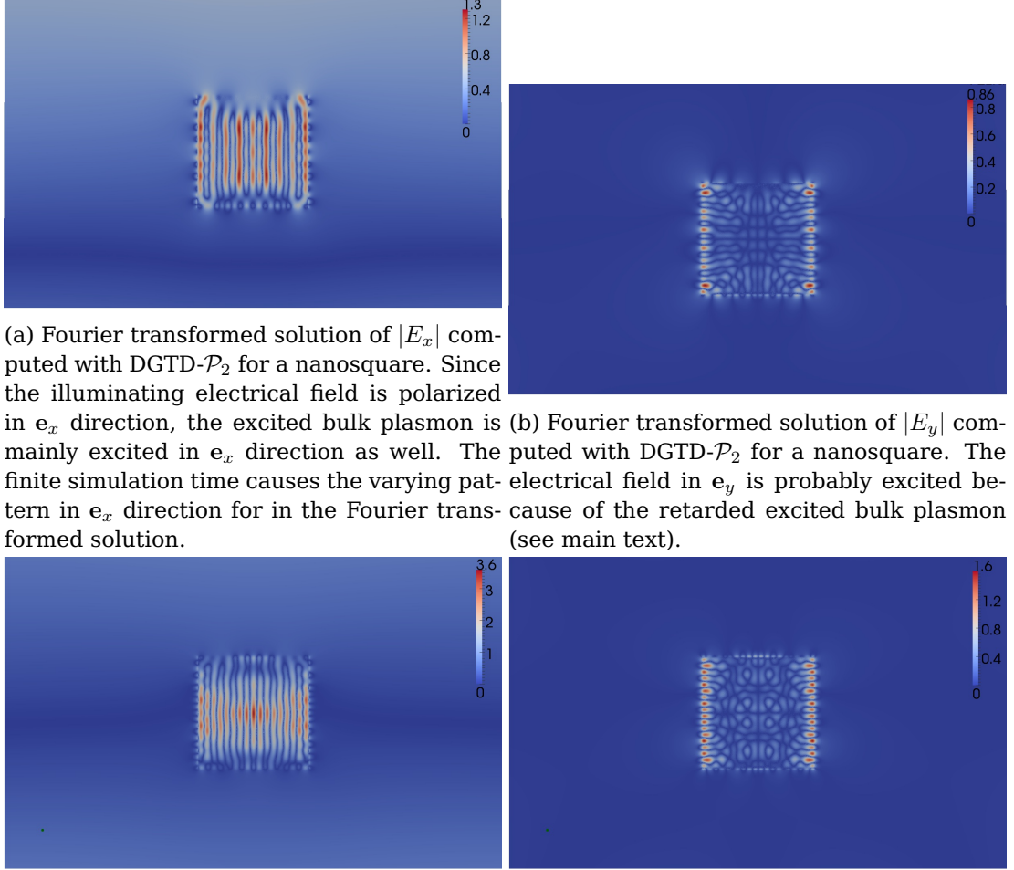
(c) Fourier transformed solution of |E_x| computed with DGTD- \mathcal{P}_2 for a nanosquare. Here, the computation time is two times longer compared to Figure 16a which leads to a smoother pattern.
