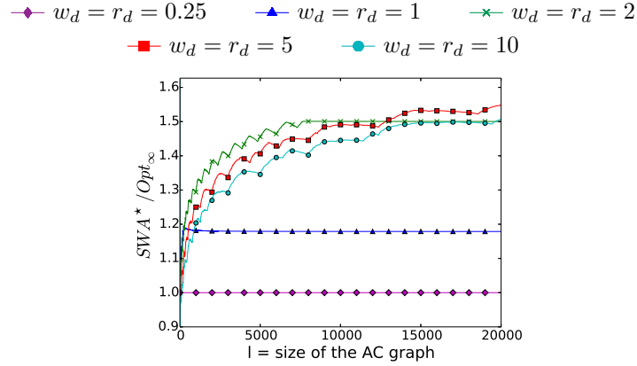
Figure 7: Ratio \text{SWA}^*(l, c_m, w_d, r_d) / \text{Opt}_\infty(l, c_m, w_d, r_d) as a function of l , for c_m = 5 .
