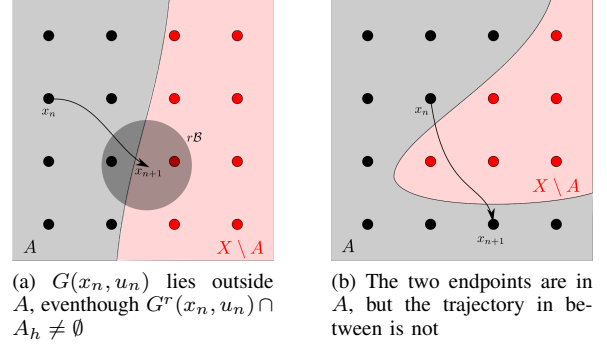
Fig. 1: Algorithm Issues
