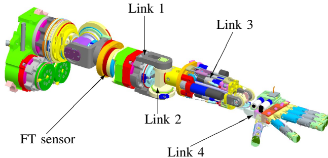
Fig. 2. CAD drawing of the seven degree-of-freedom iCub arm used in the experiments. Three out of the four joints (two in the shoulder and one in the elbow) are sensorized with joint level torque sensors. These joints are the one considered in the proposed experiments.
