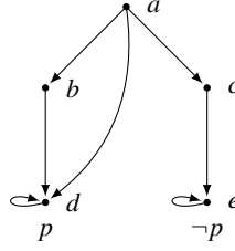
Fig. 1. Model for example formula with global modalities.
