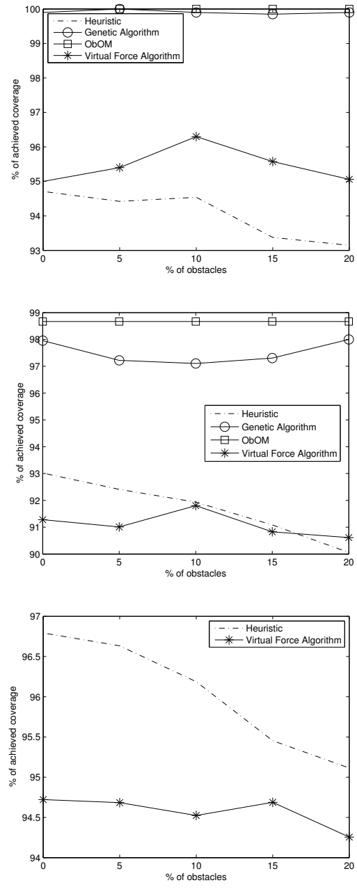
Fig. 5: Percentage of coverage when the grid size is 10 \times 10 (a) 15 \times 15 (b) and 25 \times 25 (c) and obstacles are considered.
