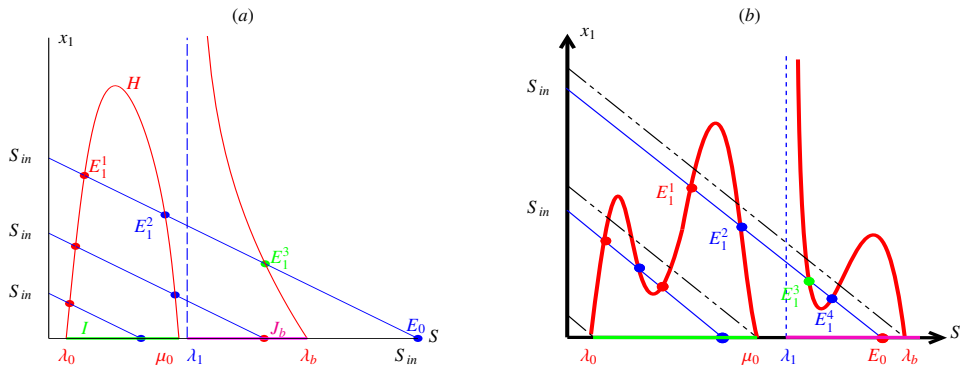
Figure 3: The case \mu_0 < \lambda_1 : Multiplicity of positive equilibria: H is decreasing (a) and non-monotonic (b) on J_b .
