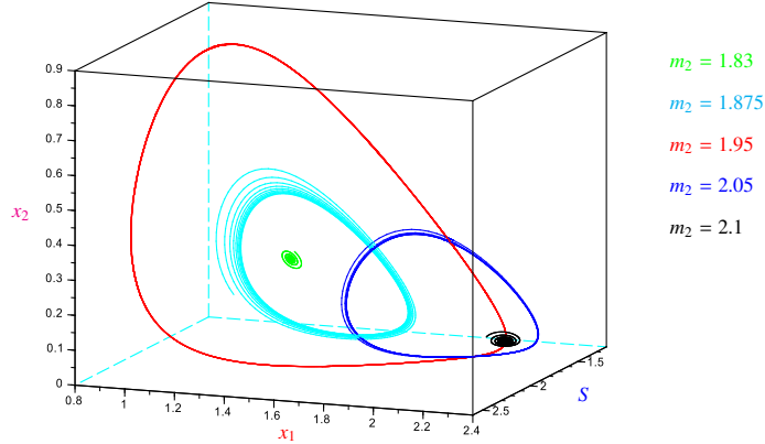
Figure 13: Occurrence and disappearance of limit cycles in the three-dimensional space (S, x_1, x_2) for different values of m_2 .
