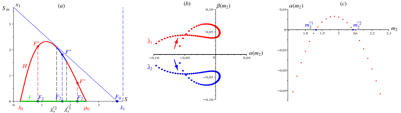
Figure 10: (a) Change of asymptotic behavior for S_{in} > \bar{S}_{in} and \lambda_2 \in I . Double super-critical Hopf bifurcation: Variation of a pair of complex-conjugate eigenvalues (b) and the corresponding real part (c) as m_2 increases.
