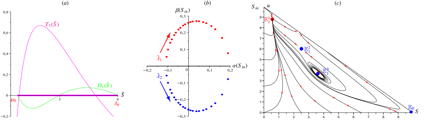
Figure 4: Sub-critical Hopf bifurcation: (a) change of sign of T_1(\bar{S}) where D_1(\bar{S}) > 0 . (b) Variation of a pair of complex-conjugate eigenvalues as S_{in} increases. (c) The phase portrait of (12) for S_{in} = 9.95 .
