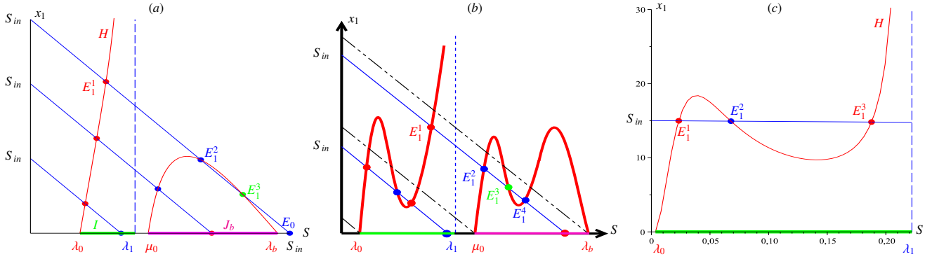
Figure 2: The case \lambda_1 < \mu_0 : Multiplicity of positive equilibria: H is increasing (a) and non-monotonic (b) on I . (c) Numerical example of existence of three positive equilibria.
