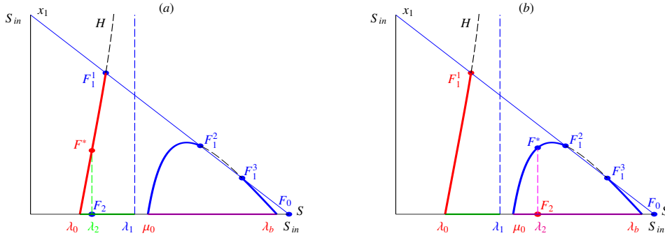
Figure 6: When \lambda_1 < \mu_0 : Case a: \lambda_2 \in I ; Case b: \lambda_2 \in J_b .
