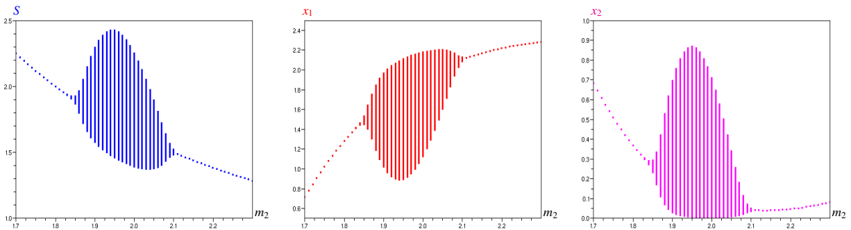
Figure 11: Projections of the \omega -limit set in coordinates S , x_1 and x_2 depending on m_2 : Occurrence and disappearance of limit cycles through a double super-critical Hopf bifurcation.
