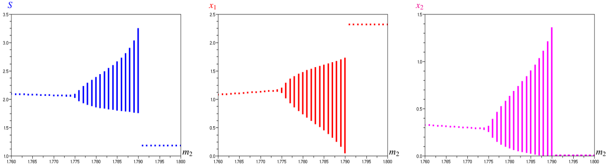
Figure 8: Projections of the \omega -limit set in variables S , x_1 and x_2 , as a function of m_2 , reveal the occurrence of limit cycles through a super-critical Hopf bifurcation and disappearance through a homoclinic bifurcation.
