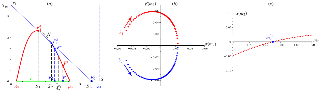
Figure 7: (a) Change of stability: F^* is LES on the red curve and unstable on the blue curve. Variation of a pair of complex-conjugate eigenvalues (b) and the corresponding real part (c) as m_2 increases.
