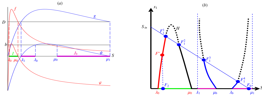
Figure 15: (a) Interval of existence of equilibria F_1 and F^* in the case \mu_0 < \lambda_1 . (b) Existence of a unique positive equilibrium F^* .
