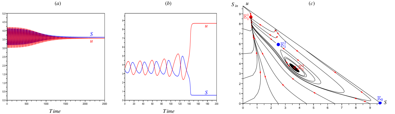
Figure 5: Bi-stability of \mathbb{E}_1^3 and \mathbb{E}_1^1 for S_{in} = 9.8 .
