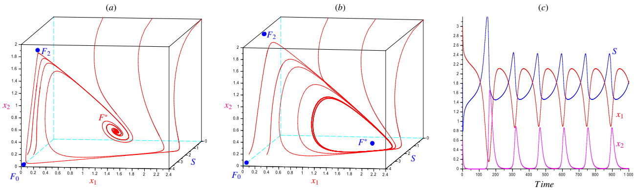
Figure 12: Coexistence: global convergence to the positive equilibrium F^* or to the limit cycle.
