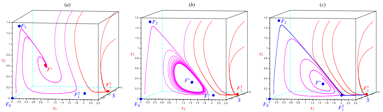
Figure 9: Super-critical Hopf bifurcation and homoclinic bifurcation: bi-stability, coexistence and limit cycle.
