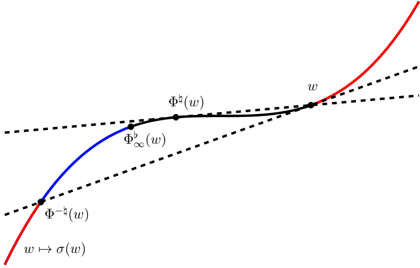
Figure 1: Notations used for solving the Riemann problem. \Phi^{-b}(w) is the first Liu shock reachable from w . The entropy dissipation between w and \Phi_\infty^b is zero. The states in red can be linked to w by a Liu shock, the blue ones by a nonclassical shock.
