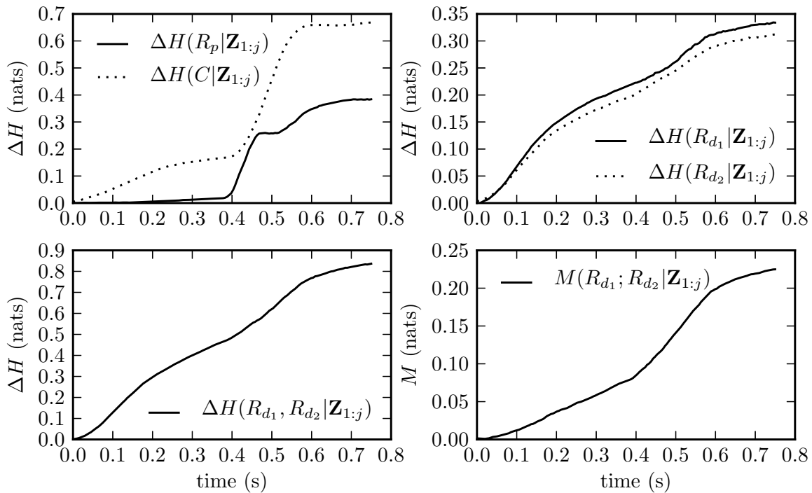
Figure 6: Mutual information between R_{d_1} and R_{d_2}
