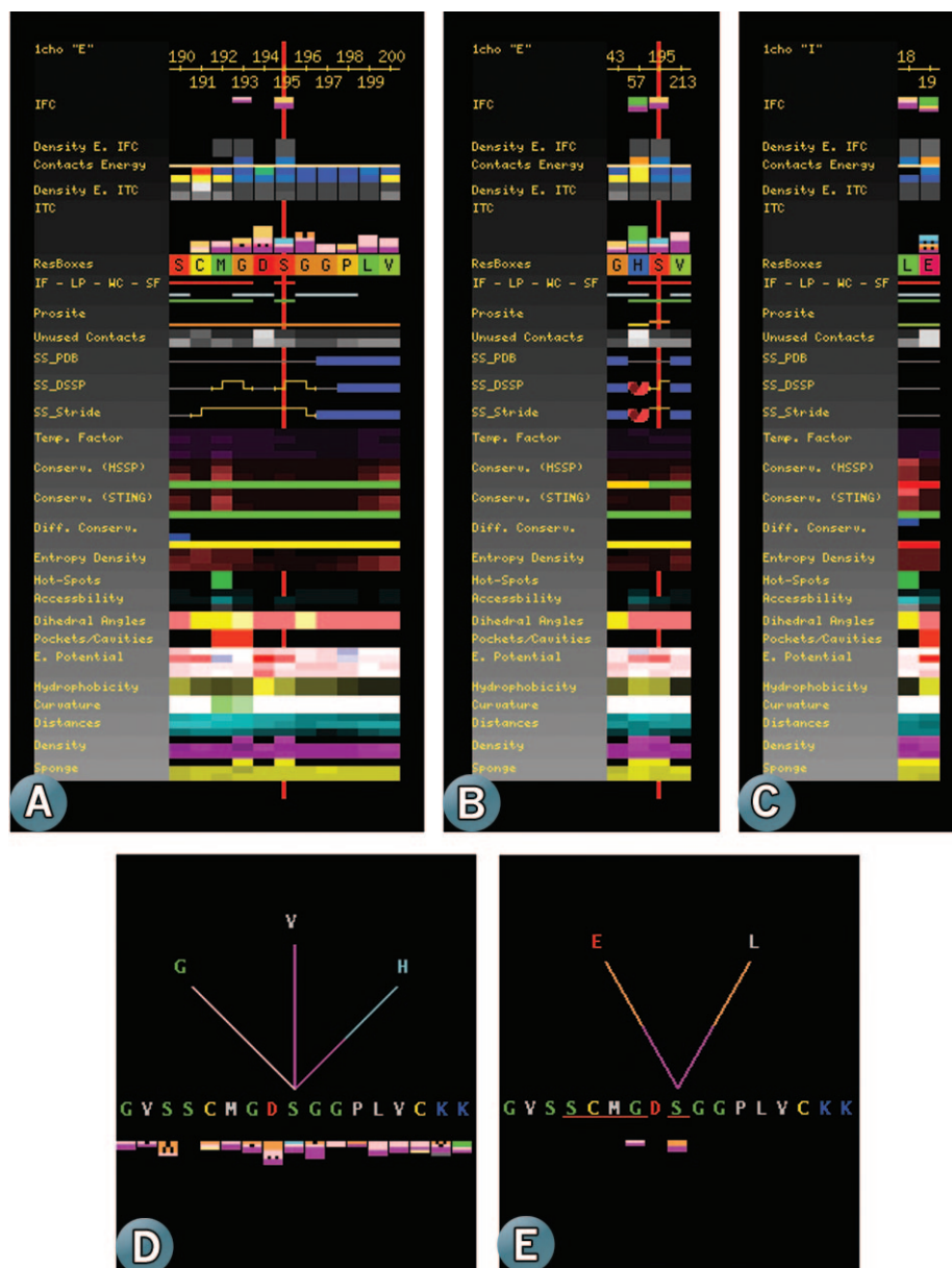
Figure 1. The STING Report J PD image area contains three distinct images (data taken for the 1cho.pdb file, chain E, residue Serine_195): (A) this image shows all parameters for a sequence of 11 residues with the selected Serine_195, at the central position; (B) this image shows the Serine_195 residue plus all residues of the same chain, making the inter-atomic contacts with it; and (C) this image shows all residues belonging to the 'I' chain which is different from the one where the selected residue is located (chain 'E') and which make the inter-atomic contacts across formed interface. By quick inspection of the J PD shown parameters, one can see that the conservation is very high for a number of residues (dark boxes at the Conservation row), including Serine_195. In addition, one can observe that the Serine_195 makes internal contacts with three other amino acids, one of them being His_57, also a member of the catalytic triade. The Graphical Internal (D) and Interface Forming Residue (IFR) Contacts (E) images show the fan-like representations of the amino acids inter-atomic contacts established with the Serine_195. The color coding of the virtual contacting lines follows the established color code in STING Millennium Suite (SMS) (2). The color code practiced here is also self evident from the Figure 2. (A) The Java Table of Contacts ( J TC) image is presented. Note that not all the red underlined residues (belonging to the interface) are actually making the IFR contacts.
