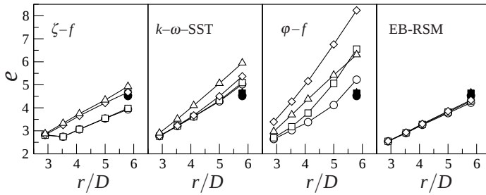
Figure 9. Radial evolution of entrainment ratio e for \omega D/U_j = 0.00 (○); 0.12 (□); 0.24 (△); 0.48 (◇). Filled symbols: Experiments.
