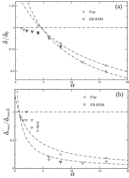
Figure 6. Scaling with \alpha of (a) \delta/\delta_0 and (b) \delta_{\max}/\delta_{\max 0} . Lines: theoretical relations fitted to the experimental and numerical results.
