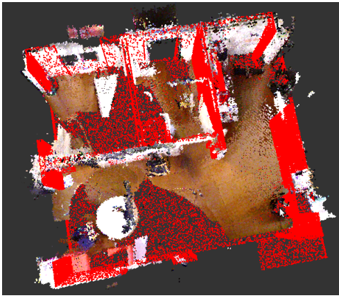
Fig. 9. The superposition of a 3D model (only ground and walls displayed in red) with the map obtained by the SLAM.
