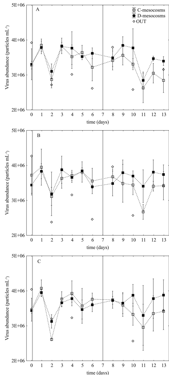
Figure 6. Virus abundance (particle \text{mL}^{-1} , mean \pm standard deviation of three replicate mesocosms) in D- and C-mesocosms and OUT samples at surface (a), 5 m (b) and 10 m (c) depth during the DUNE-R experiment. Grey vertical bars represent the dust seedings.
