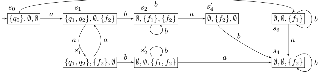
■ Figure 2 The IA-automaton of pLTS depicted on the right of Figure 1.
