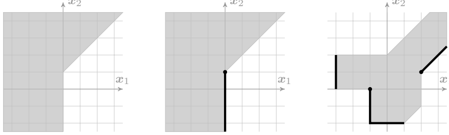
Fig. 3. Tropical polyhedra with mixed constraints (the ends of the black segments marked by points are included in the polyhedra).
