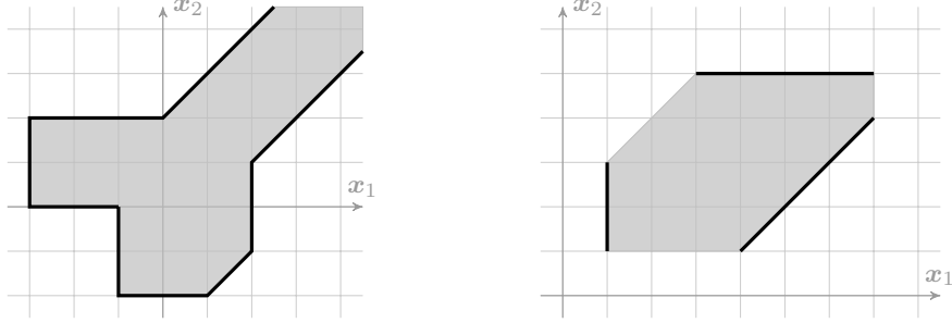
Fig. 1. Left: a tropical polyhedron (including the black border). Right: a (non-closed) zone defined by the inequalities 1 \leq x_1 < 7 , 1 < x_2 \leq 5 , -2 < x_1 - x_2 \leq 3 .
