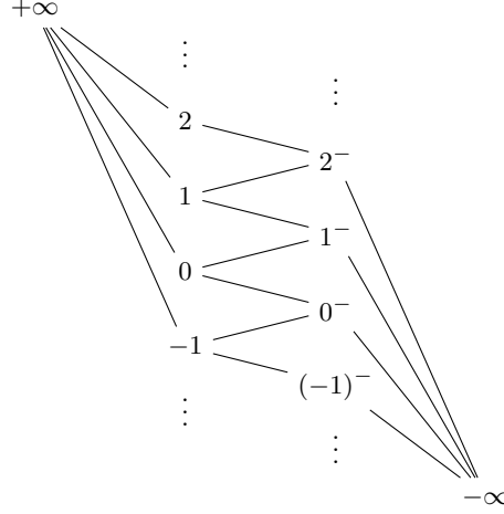
Fig. 2. Hasse diagram of the order \leq_{\mathbb{G}} over the elements of \mathbb{G} with modulus in \mathbb{Z} \cup \{\pm\infty\} .
