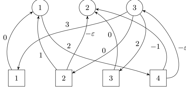
Fig. 5. The digraph associated with a parametric mean payoff game (column and row nodes are respectively represented by circles and squares).
