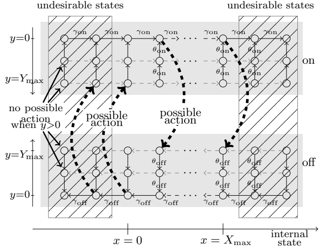
Figure 1: Markov model of an appliance. Each state is characterized by a tuple (s, x, y) , with s \in \{\text{on}, \text{off}\} . The x -axis represents the internal state ( e.g. , temperature). The y -axis is the time before the device can be switched on or off.
