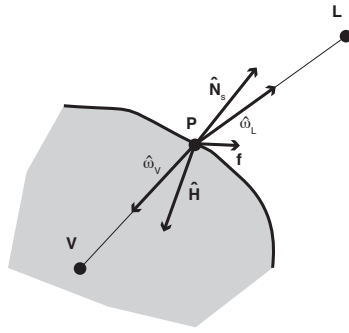
Figure 3: At point P , we define the half-vector \widehat{\mathbf{H}} , and compare it with the shading normal \widehat{\mathbf{N}}_s . Our goal is to find zeros of the function \mathbf{f} = \widehat{\mathbf{H}} + \widehat{\mathbf{N}}_s .
