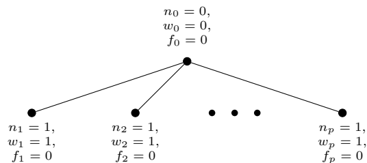
Figure 5: Tree used for the proof of Lemma 2.
