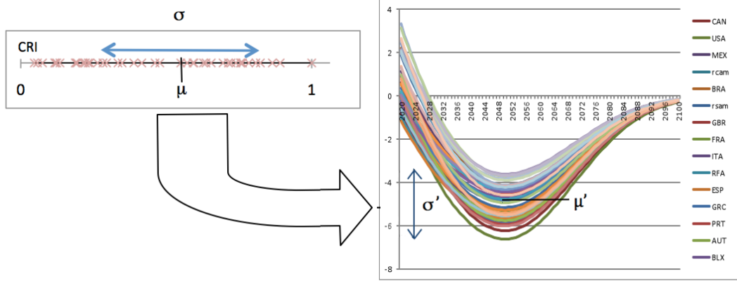
Figure 1: Parameterization the maximum effort for each of the countries with its CRI.
