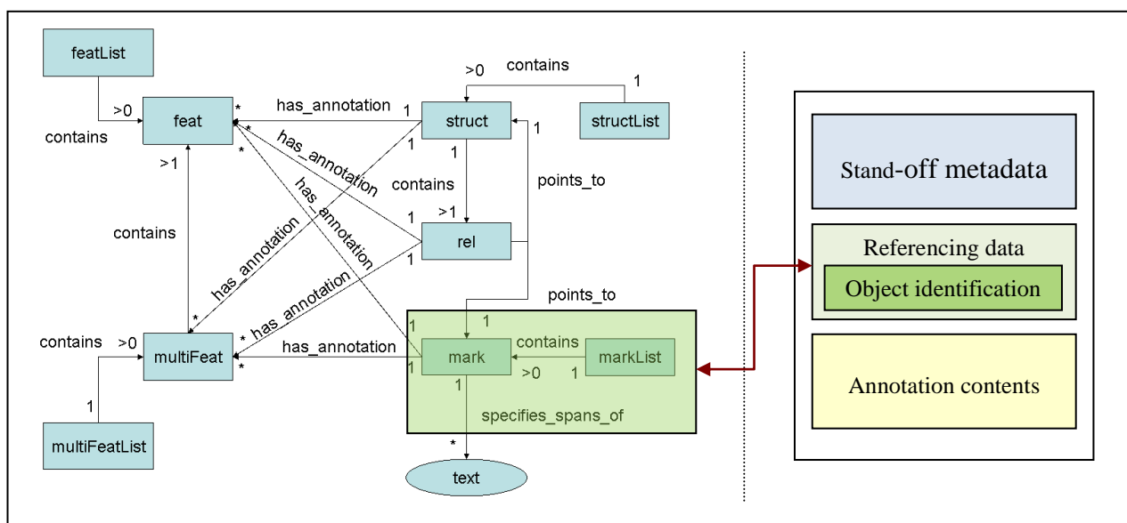
Fig. 4: Paula 1.0 Conceptual Structure (Data Model) with <multiFeat> and <...List> elements
