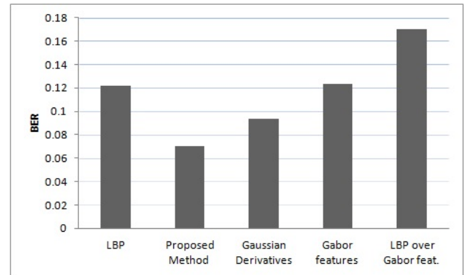
Fig. 6: BER of different descriptors over the GENKI-4K database
