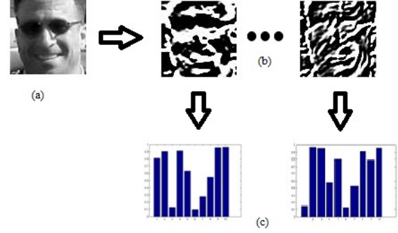
Fig. 2: Creating the features: a) original image, b) Gaussian derivative images, and c) concatenation of resulting histograms after applying LBP.
