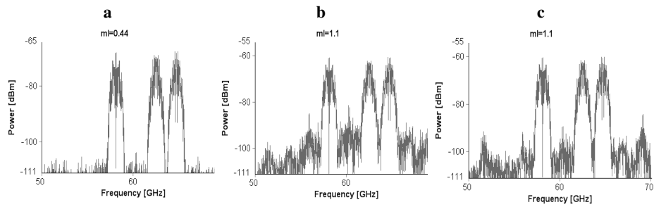
Fig. 4. Received electrical spectrum, showing intermodulation power falling on the 60 GHz channel. a) m_i=0.44 fiber length of 5 km. b) m_i=1.1 fiber length of 5 km. c) m_i=1.1 fiber length of 50 km.
