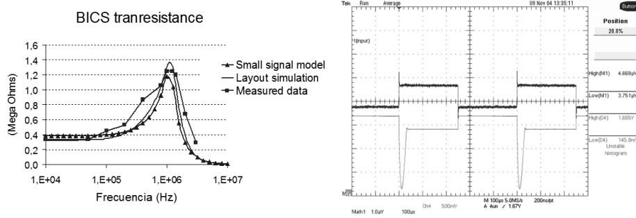
Fig. 3. BICS tranimpedance measure: (a) frequency and (b) transient responses.
