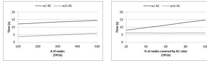
(a) Various # of nodes; AC rules Coverage: 100%. (b) Various coverage of AC rules; 500 nodes.
