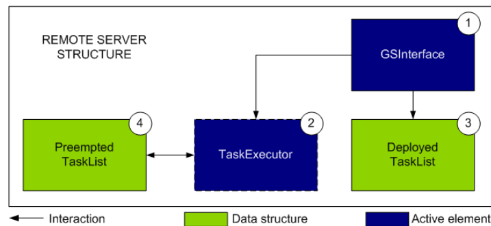
Fig. 5. Structure of the Remote Server (RS)
