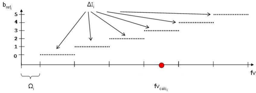
Fig. 2 Example of backward calculation (reverse mapping) of a feature vector element f_{v_{calc,i}} based on the corresponding reference BioHash b_{ref,i} , Interval Length \Delta I and Interval Offset \Omega_i .
