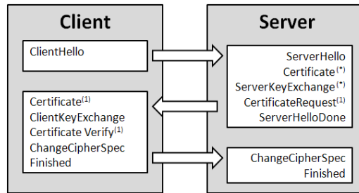
Fig. 1: The TLS Handshake Protocol
