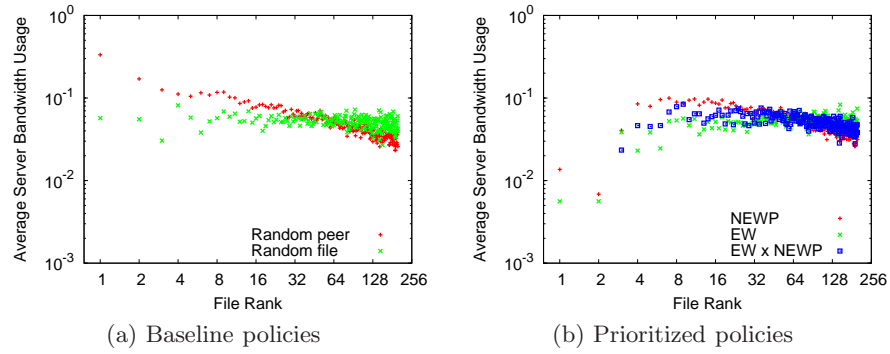
Fig. 3. Server bandwidth usage ( B = 10 , \lambda_i = 40/i , L = 1 , U = 1 , D/U = 3 , K = 256 , N = 200 )
