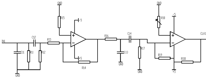
Fig.2: Circuit schematic diagram of single channel
