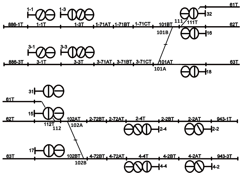
Fig. 1. Signalling layout of the Panthong Station (double track)
