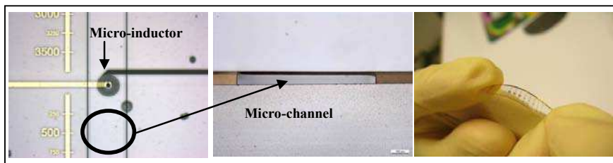
Figure 11. Photographs of the flexible integrated microsystem with SU-8 microfluidic network
