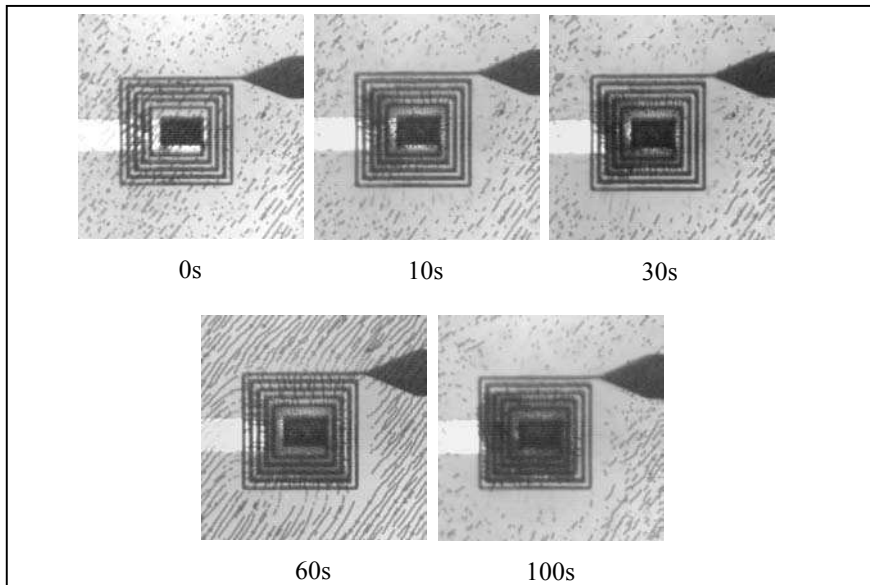
Figure 16. Magnetic beads trapping using our microelectromagnets. (0s) without excitation applied. (10s to 100s) after excitation ( I=50mA ) applied to the microelectromagnet: trapping beads.
