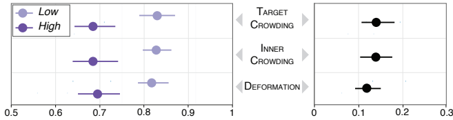
Fig. 4. Mean ACCURACY and mean ACCURACY difference as a function of task complexity for the ID tracking task. Error bars are 95% CIs.
