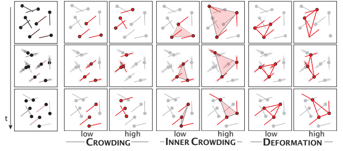
Fig. 1. Illustration of the complexity measures.
