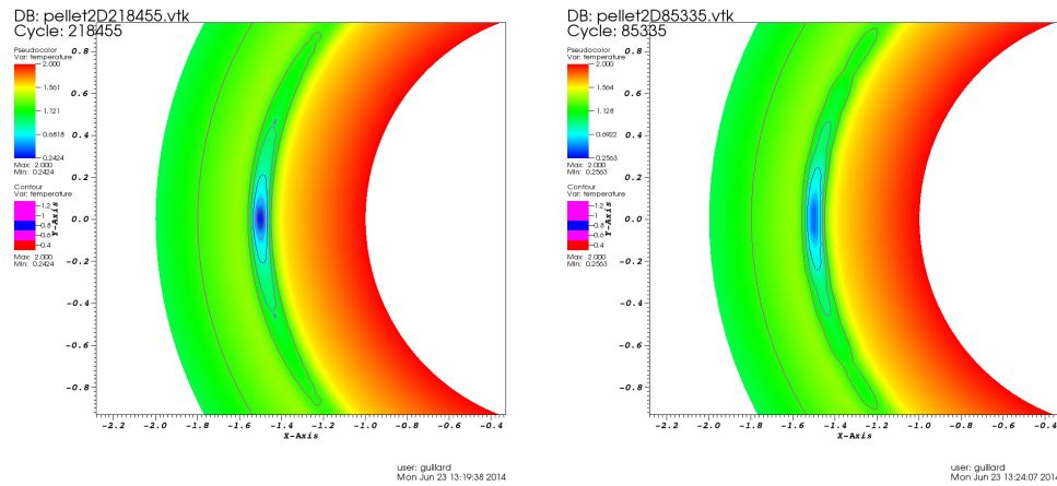
Figure 14: Left : Standard Fourier with 256 modes, Right : Mapped Fourier with 32 modes
