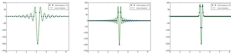
Figure 4: Fourier Interpolant of the RHS of equation 1
