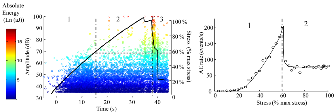
Figure 4 : (a. left) Amplitude and energy of the AE signals and stress curve. (b. right) AE rate versus stress
