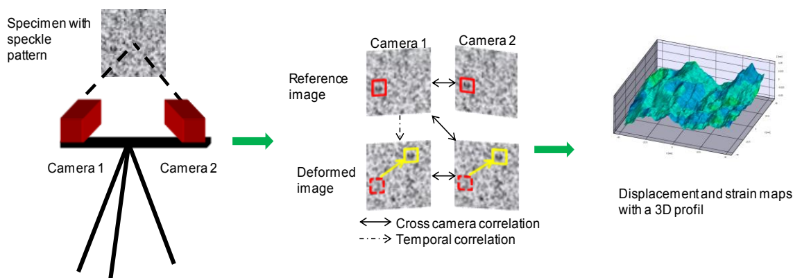
Figure 2 : Schematic view of the process of DIC
