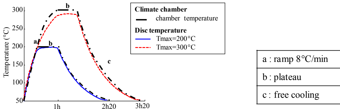
Figure 7 : Thermal cycles
