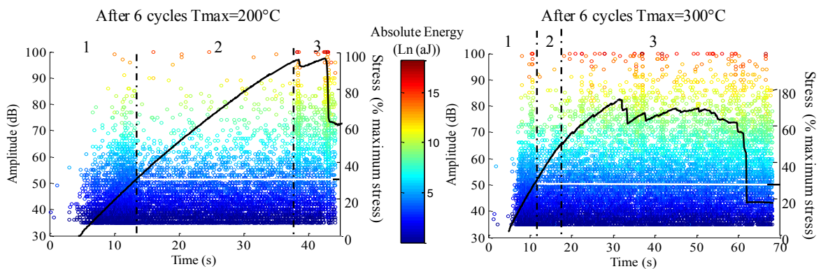
Figure 9 : Amplitude and energy of the AE signals with the stress curve of the 200°C and 300°C cycled specimens respectively.
