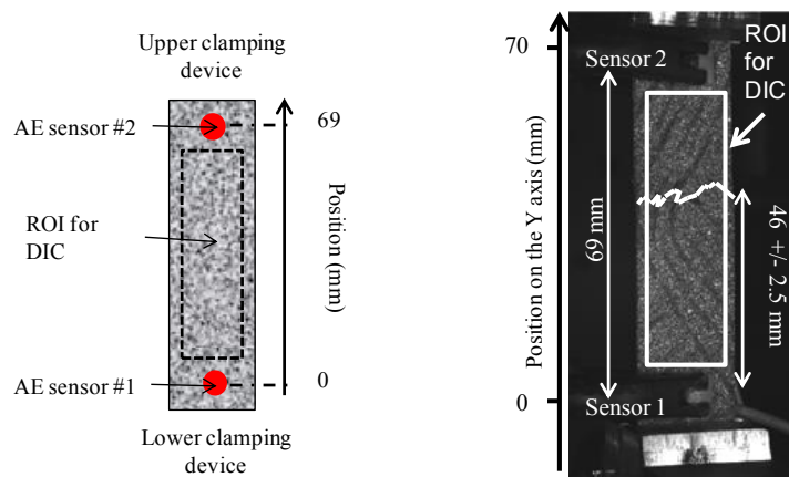
Figure 5 : Position of the two AE sensors and the region of interest (ROI)
