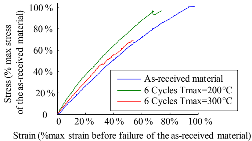
Figure 8 : Stress-strain curves for the as-received and thermally cycled material. Displacement rate 1mm/min
