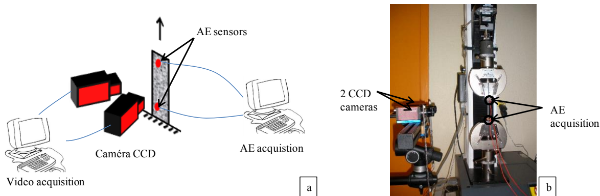
Figure 3 : Outline of the experimental set up (a) and photo (b)
