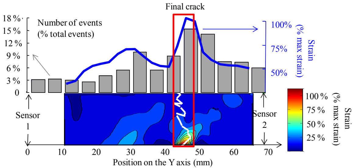
Figure 6 : Cumulative number of acoustic events and strain field prior to failure.
