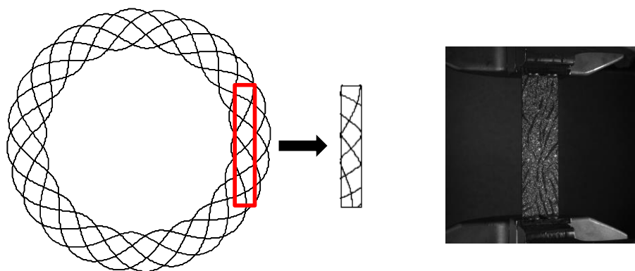
Figure 1 : Preform and view of the rectangular specimen cut into the disc.
