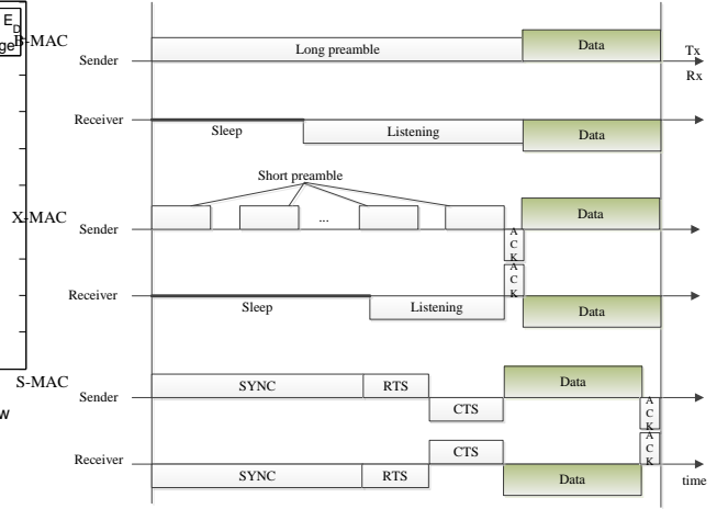
Figure 6: Schematic comparison of the timelines between B-MAC, X-MAC and S-MAC
