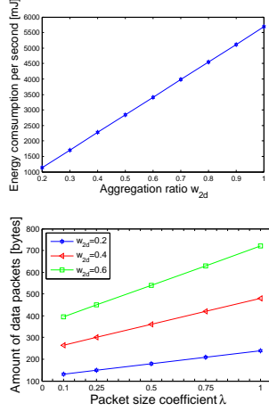
Figure 4: Energy consumption and network capacity considering with different aggregation ratio w_{2d} and packet size coefficient \lambda in 2D network
