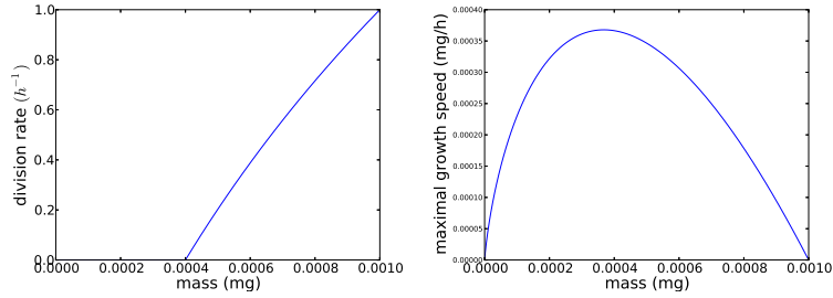
Figure 1: ► (Left) Division rate function \lambda(x) defined by (15) with \bar{\lambda} = 1 \text{ h}^{-1} , m_{\text{div}} = 0.0004 \text{ mg} and p_\lambda = 1000 . ► (Right) Maximal growth speed with the Gompertz growth speed function (14) with r_{\text{max}} = 1.0 \text{ h}^{-1} , m_{\text{max}} = 0.001 \text{ mg} (namely the RHS of the inequality (14)).
