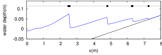
Figure 21: Cox Experience - Snapshot of the water depth profile during the breaking process. Areas in need of limiting are specified along the dotted line.
