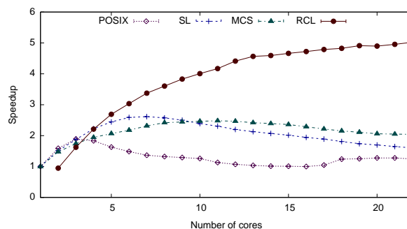
Fig. 10: Memcached/Set speedup.
