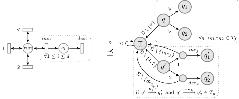
FIGURE 6. Reducing AVASS state reachability to a simulation BPP \geq FS.
