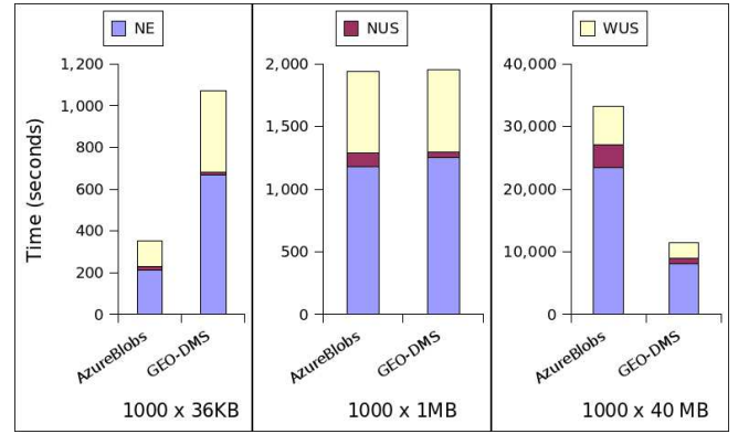
Fig. 10. Execution times of the A-Brain application across 3 datacenters, using AzureBlobs and GEO-DMS as a transfer backend. The bar indicate the total time of transferring the files towards the Meta-Reducer located in NUS
