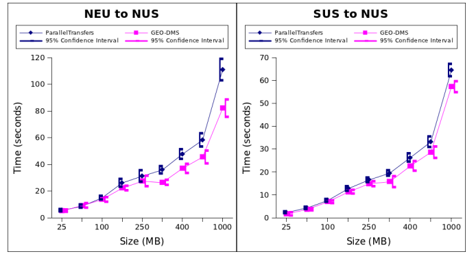
Fig. 7. Our approach (GEO-DMS) vs. simple parallel transfers. The result show the average and the 95% confidence intervals for the transfer time
