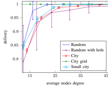
Fig. 4. Delivery ratio for Greedy routing.
