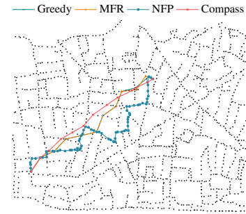
Fig. 2. City topology with an example of route.
