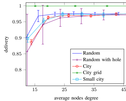
Fig. 7. Delivery ratio for Compass.
