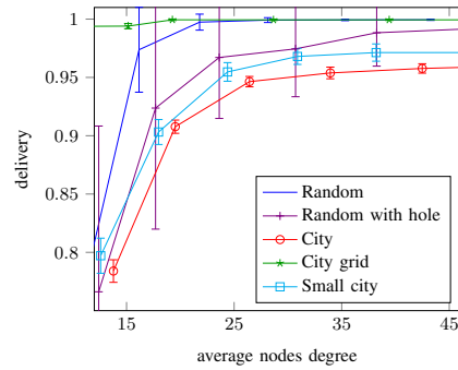
Fig. 5. Delivery ratio for NFP.
