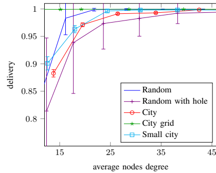
Fig. 6. Delivery ratio for MFR.
