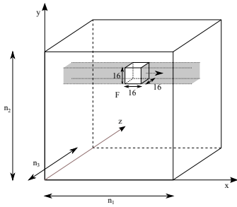
Fig. 1. 3D Convolution
