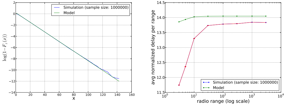
(a) Cumulative distribution in the form: \log(1 - F(x)) (b) Convergence to asymptotic expression (magnified: y-axis does not start from 0)
