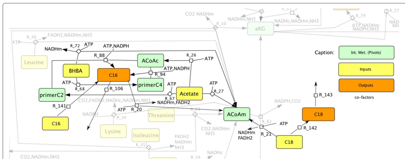
Figure 3 Modeling long-chain fatty acids oxidation (LCFA) in tricarboxylic acid (TCA) cycle. Introducing LCFA (C16:0), C(18:0)) oxidation in the TCA cycle may be required to consistently model the response to several treatments, such as the (HB) dataset (Table 1). In this case, the model shown in Figure 2 is extended by introducing inputs of C(16:0) ( R_{141} ) and C(18:0) ( R_{142} ), and output of C(18:0) ( R_{143} ). C(16:0) oxidation ( R_{20} ) and C(18:0) oxidation ( R_{21} ) are modified accordingly.
