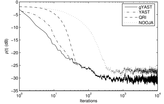
Fig. 3. Subspace Tracking
