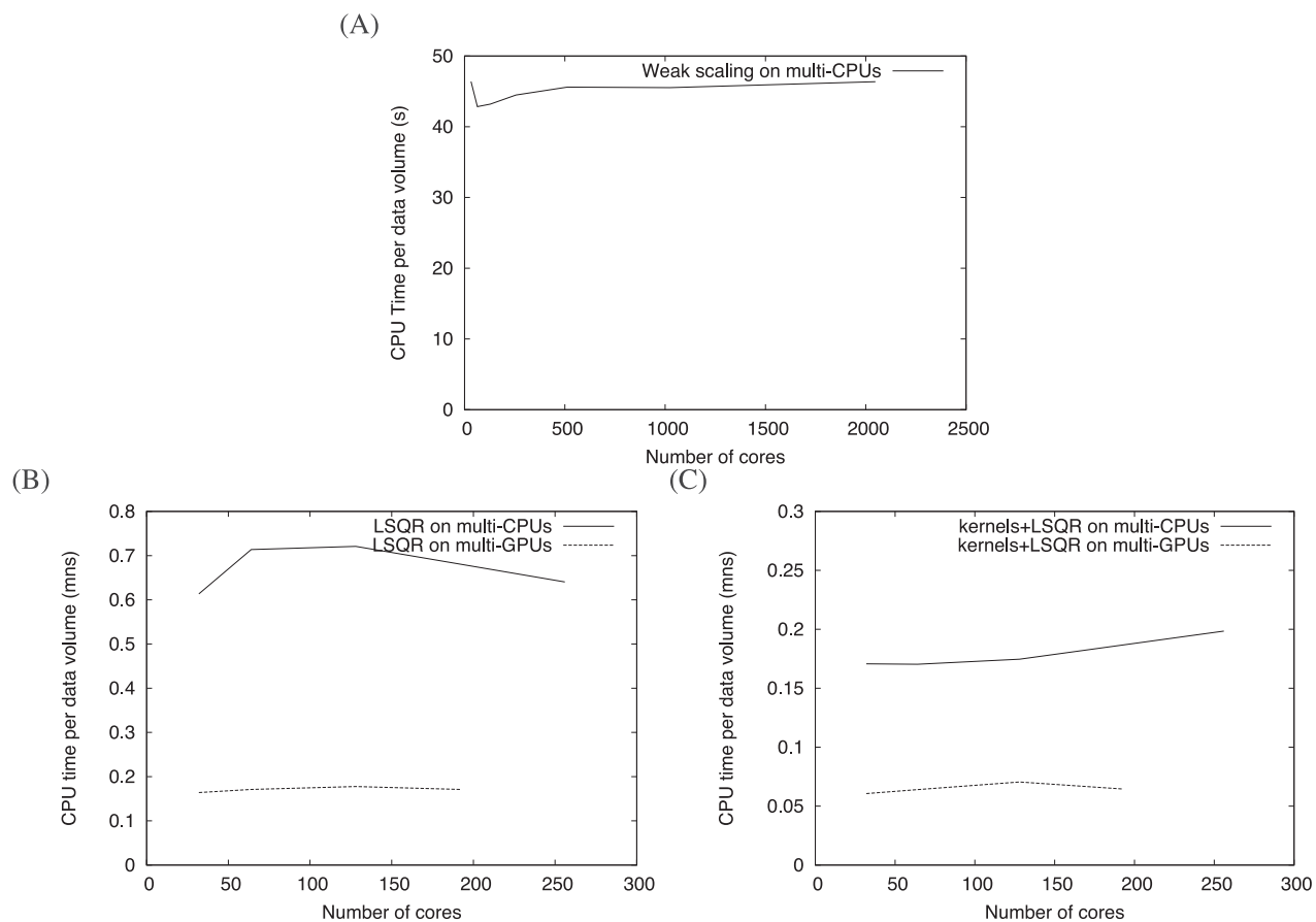
Figure 17. Weak scaling of the inversion process obtained on the multi-CPU (A) cluster. For multi-CPU we used 1500, 3000, 6000, 12 000, 24 000, 48 000 and 99 856 data on, respectively, 32, 64, 128, 256, 512, 1024 and 2048 processes. We observe that scaling has a behaviour close to constant with few fluctuations. In (B) and (C) we compare the weak scaling of multi-CPU to that of multi-GPU for the whole code (kernels calculations, compression and inversion) as well as for the inversion phase only. We test 1500, 3000, 6000 and 9000 data for 32, 64, 128 and 192 for both CPU cores and GPUs. We also observe good weak scaling for multi-GPUs. GPUs accelerate the code by a factor between 4 and 5 for the whole code and around 3 for the inversion phase only.
