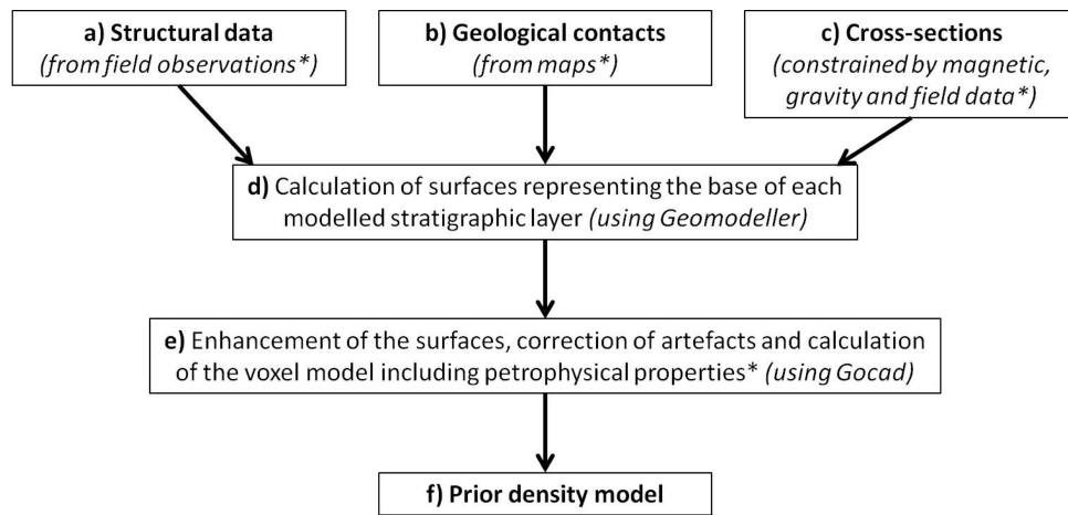
Figure 9. Simplified diagram illustrating the steps used to build the Ashanti Belt prior model: (a) field structural data (Perrouty et al. 2012), (b) geological contacts from maps and (c) cross-sections constrained by geophysical and petrophysical data were used to calculate the interfaces between the geological units (d) with Geomodeller. These surfaces were then tidied up with Gocad and a voxel model was generated (e), which corresponds to the prior density model (f).
