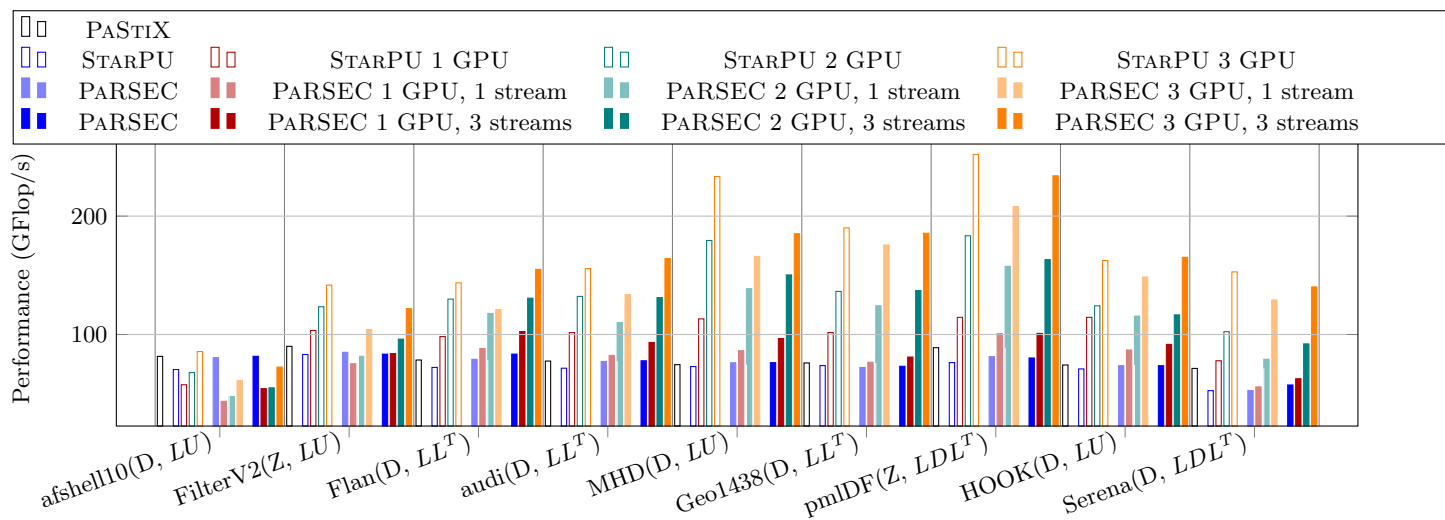
Figure 4: GPU scaling study: Flop/s reached during factorization of the different matrices, with the three schedulers, using the maximum number of cores and zero to three GPUs.
