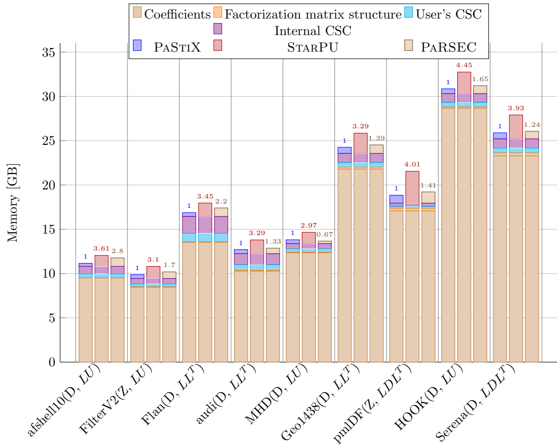
Figure 5: Memory consumption, common data structures are detailed, overhead ratio on top of bar chart
