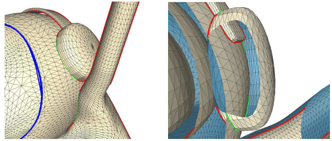
Fig. 8. Surface intersection curves (green) are common in 3D animation. This character's earmuff passes through his head; the earmuff intersects the strap; the arms intersect the hood; the skates intersect the feet; the lips intersect each other (Figure 1). Correctly handling surface intersections is crucial for accurate rendering of production geometry. Red © Disney/Pixar
