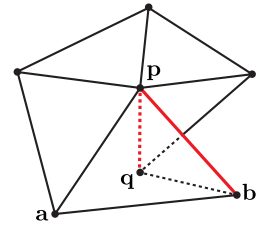
Fig. 20. A curtain-fold cusp in the contour. Edge \overline{\mathbf{pb}} is an exterior contour. Edge \overline{\mathbf{pq}} is an interior contour, indicating that it is occluded by a nearby face. Vertex \mathbf{p} is thus a curtain-Fold cusp [Markosian et al. 1997]. (A cusp of the mesh boundary curve occurs in the same configuration, but with triangle \mathbf{pqb} removed.)
