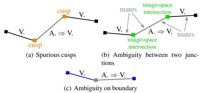
Fig. 22. Resolution of visibility ambiguities. Three heuristics are used to resolved visibility of ambiguous chains. (a) An ambiguous chain connecting two visible cusps is considered visible. (b) An ambiguous chain connecting two image-space intersections whose mates are both visible is also visible. (c) An ambiguous boundary chain connected to a visible chain not at an image-space intersection is marked visible.
