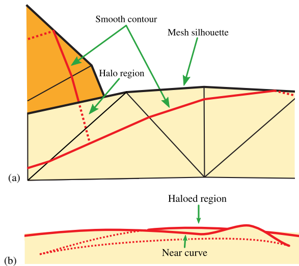
Fig. 6. Haloing problem of interpolated contours. (a) As pointed out by Eisemann et al. [2008], in image space, the interpolated contours lie inside the mesh contour, which affects planar map stylization. However, it also affects visibility, as there is a “halo region” between the two contours in which the mesh occludes any curves behind it, but the interpolated contour does not connect to the visible part. (b) An image-space illustration of highly-foreshortened curves in which the nearer curves will cause visibility errors for more distant curves. Here, the near curve’s halo hides the far curve. Situations like this often arise for surfaces with noisy, nearly-flat regions, such as the Stanford bunny.
