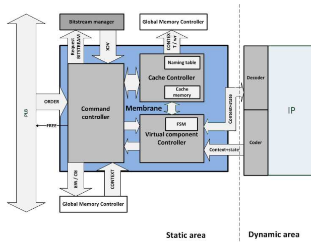
FIGURE 4 – Architecture de la membrane
