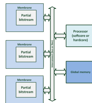
FIGURE 3 – Architecture reconfigurable à base de composants
